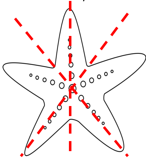
Radial Symmetry
