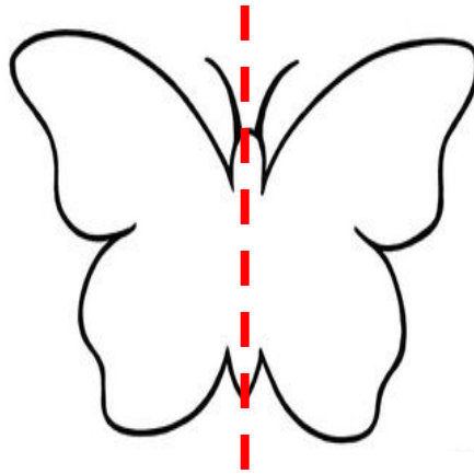
Bilateral Symmetry
