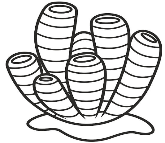
No Symmetry
