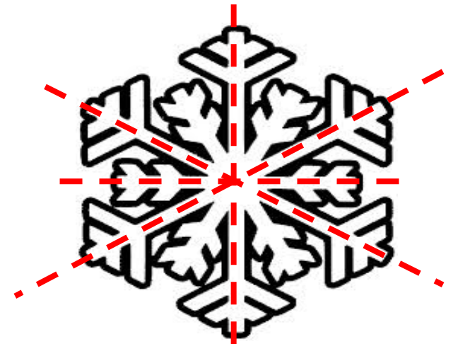
Radial Symmetry
