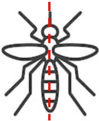
Bilateral Symmetry
